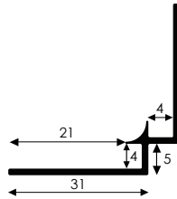
134220 Binnenhoekprofiel 4/4100 anod (+T) Internal corner 4/4100 anod (+T) Inneneckprofil 4/4100 elox (+T)
